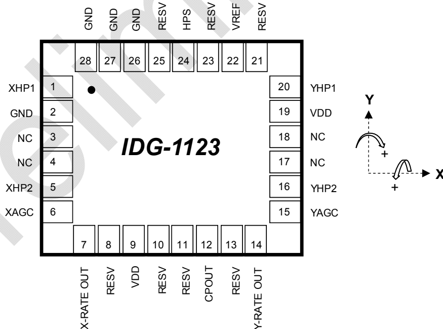
28-pin, 4mm x 5mm x 1.2mm QFN Package
